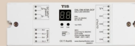
DALI LED Driver 4 CH 7A
