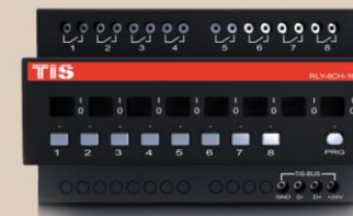
Latching Relay Module 8 Channel 20A RLY-8CH-16A
